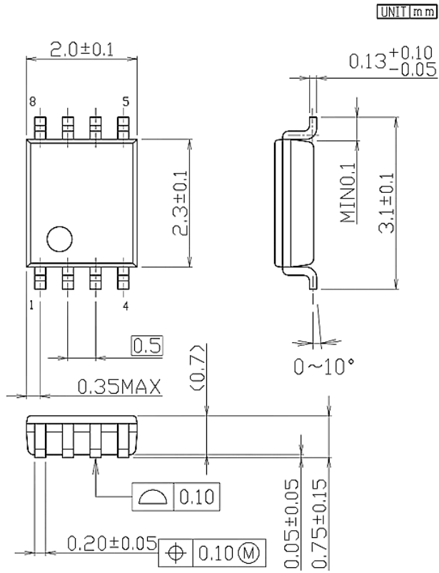
Dimensional Drawing
