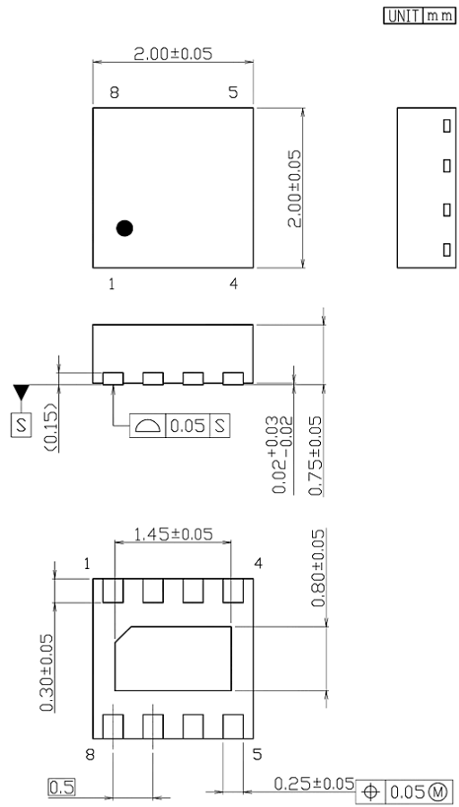
Dimensional Drawing
