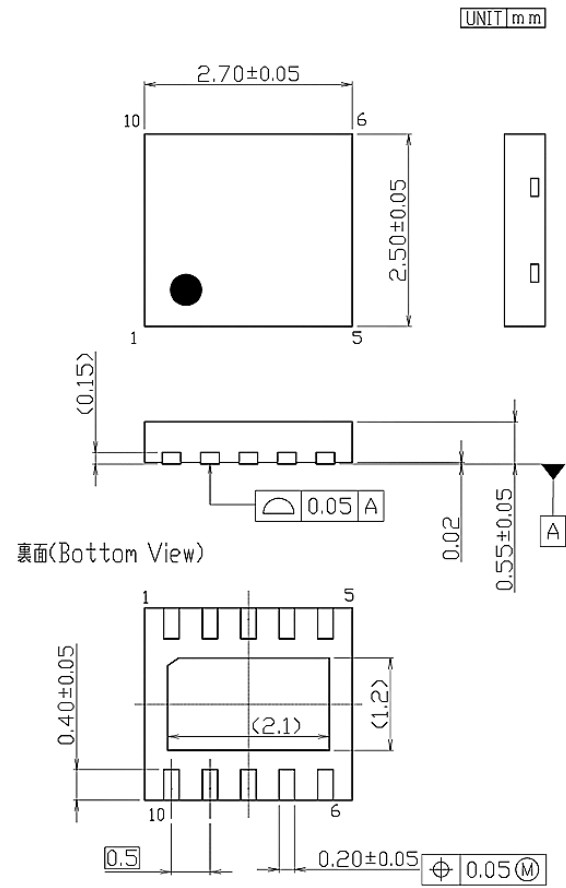
Dimensional Drawing
